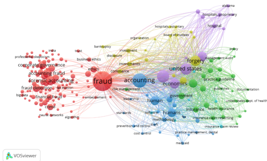
Gambar 3. Analisis Co-Accurance.
